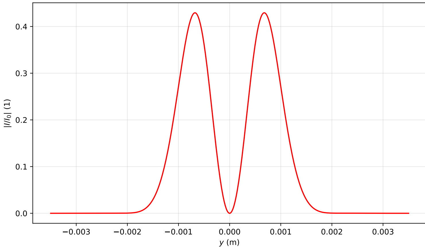
Intensity profile I(x=0, y, z=1.911)/I_0 , P_{in}=1.0P_{cr} , artificial time
